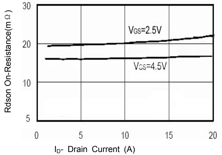
Figure 6 Drain-Source On-Resistance
